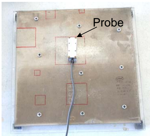
3-layer specimen with total thickness of 0.500" on top of corrosion standard
